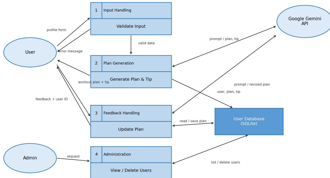
FitBuddy - Data Flow Diagram
